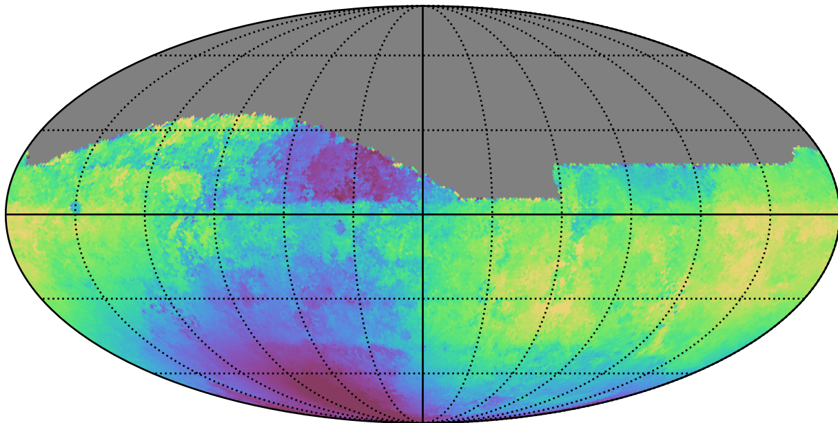
weather_cloudso20v3.4_10yrs All sky g band: Median solarElong
