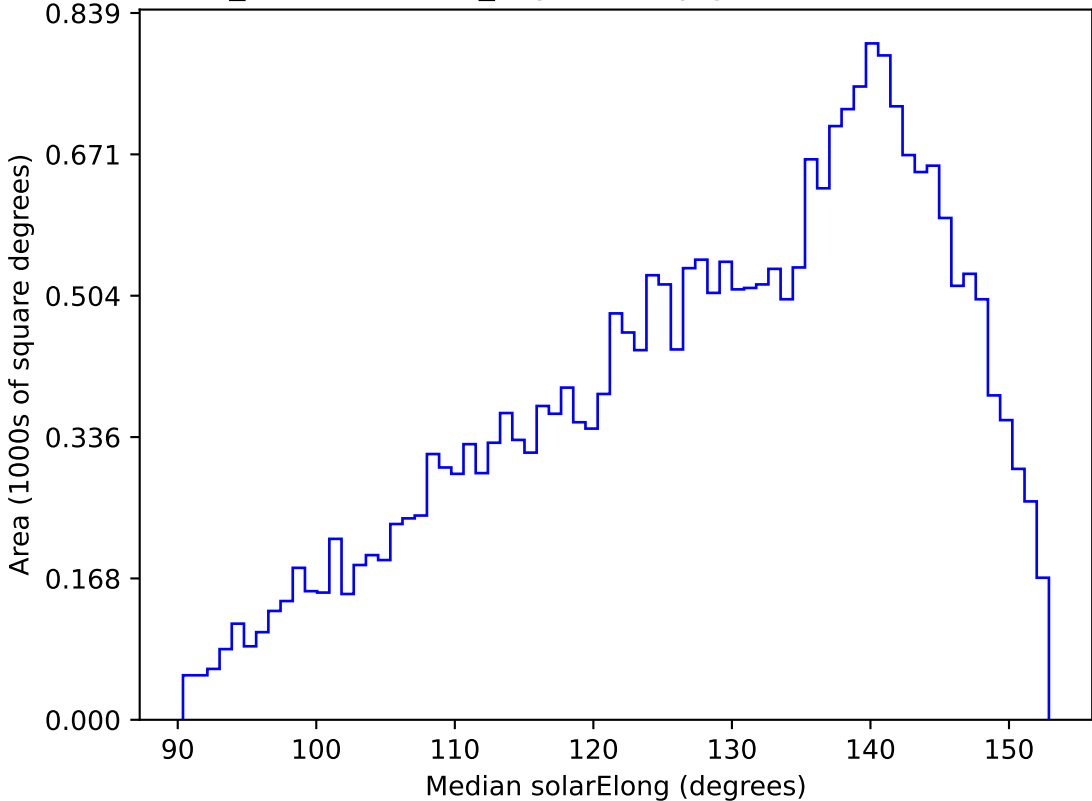
weather_cloudso20v3.4_10yrs All sky g band: Median solarElong
