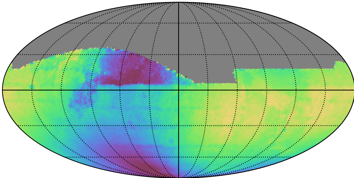
weather_cloudso20v3.4_10yrs All sky all bands: Median solarElong
