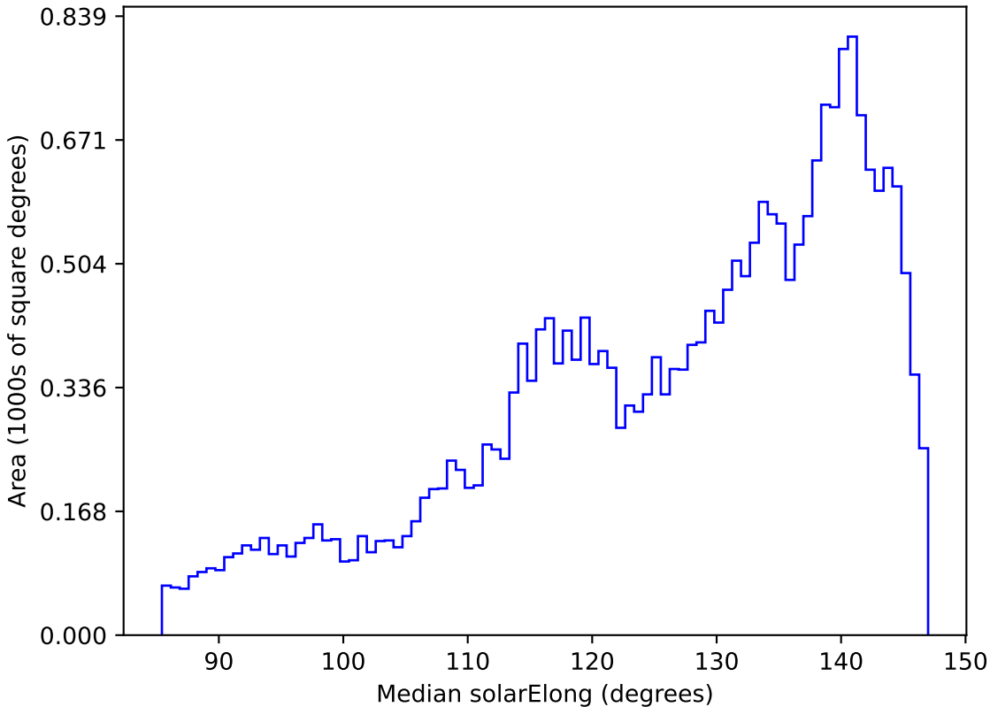
weather_cloudso20v3.4_10yrs All sky all bands: Median solarElong
