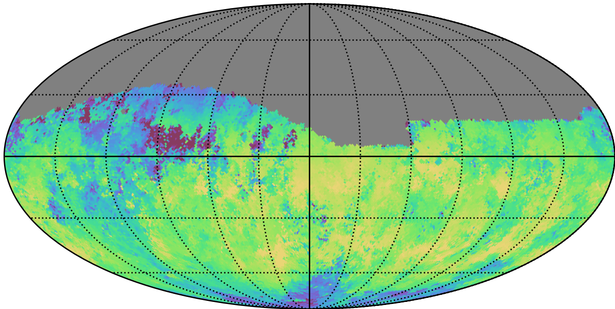
weather_cloudso20v3.4_10yrs Yr 1 z band: Median skyBrightness
