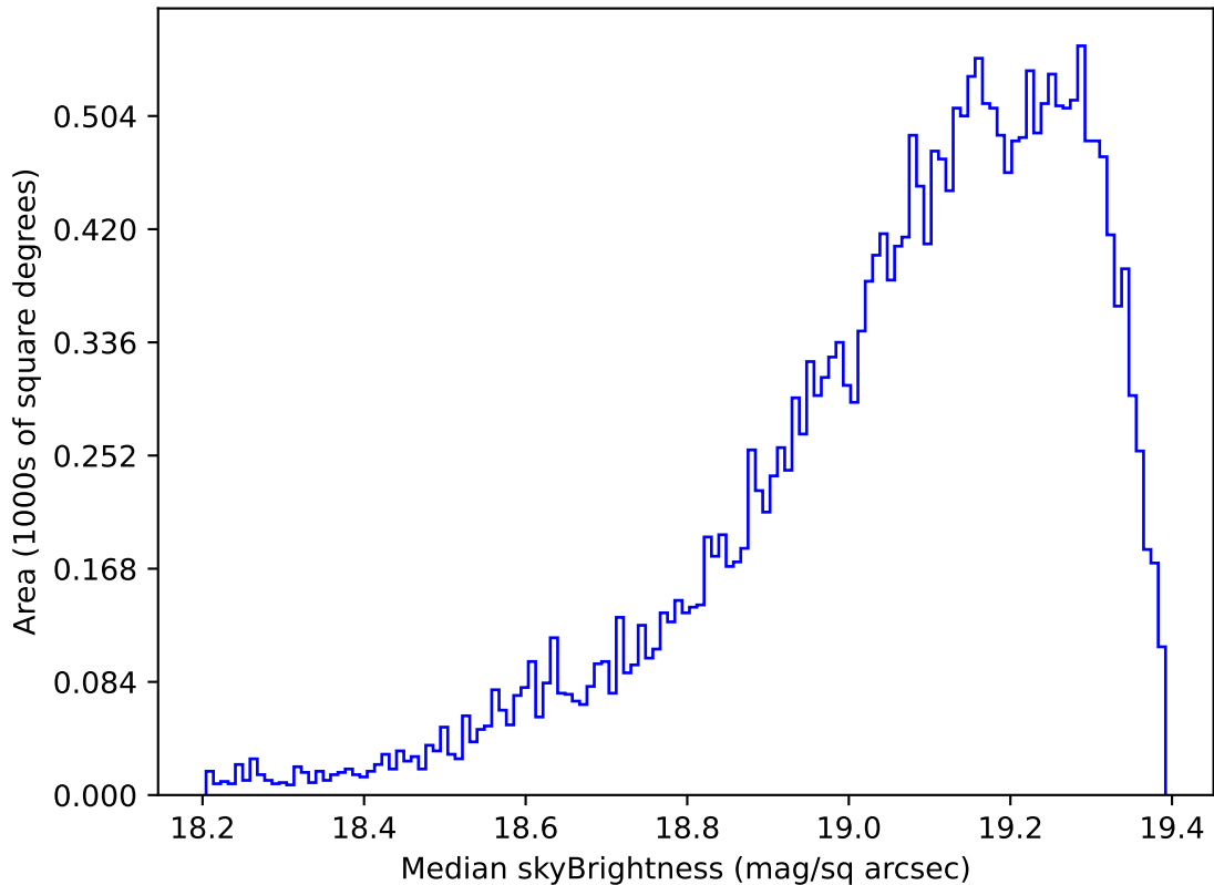
weather_cloudso20v3.4_10yrs Yr 1 z band: Median skyBrightness
