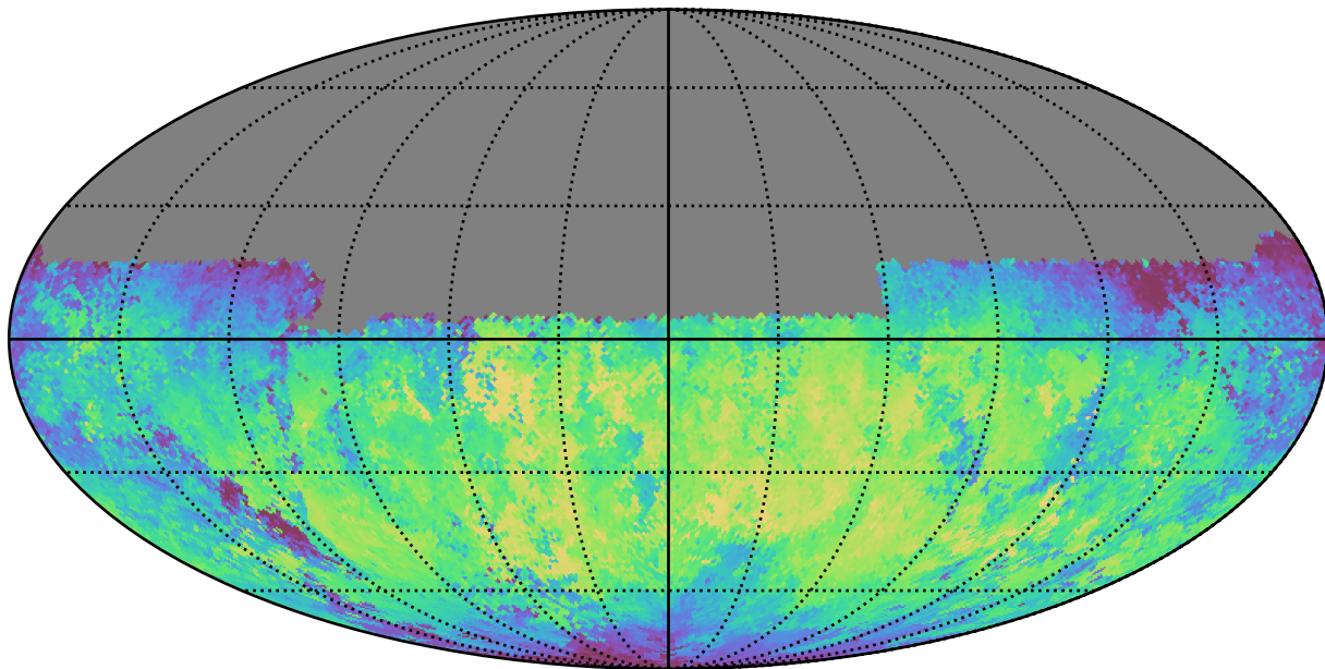
weather_cloudso20v3.4_10yrs Yr 1 y band: Median skyBrightness
