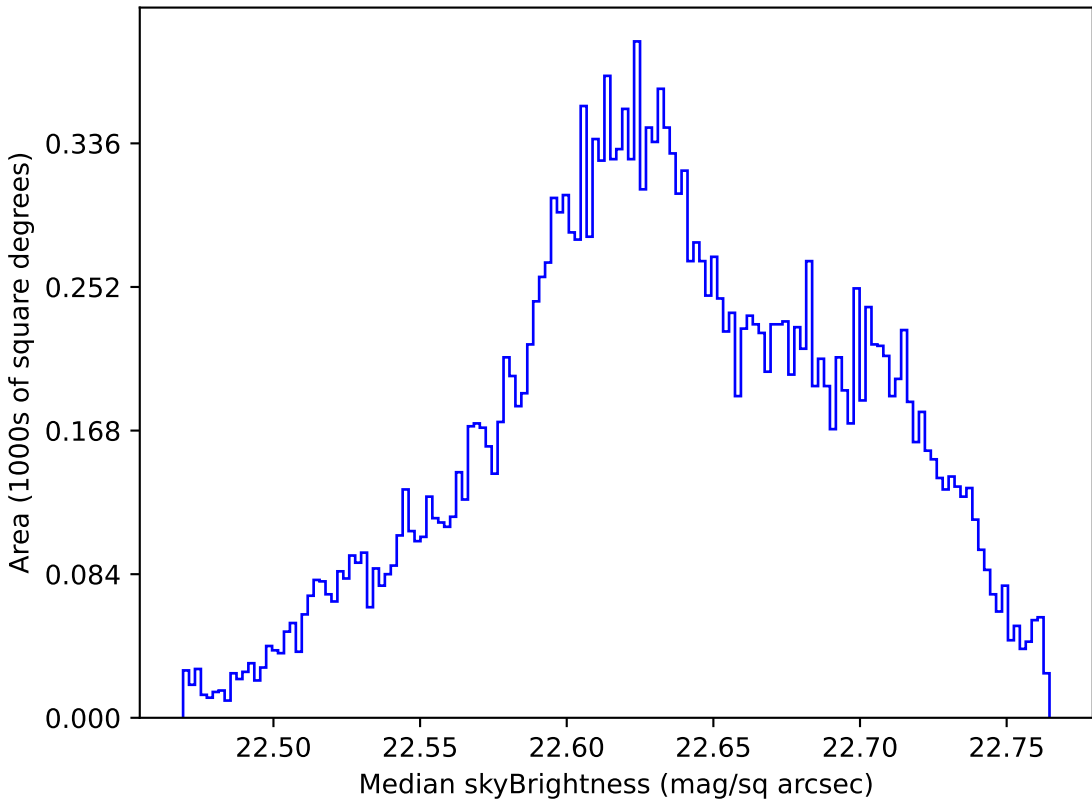
weather_cloudso20v3.4_10yrs Yr 1 u band: Median skyBrightness
