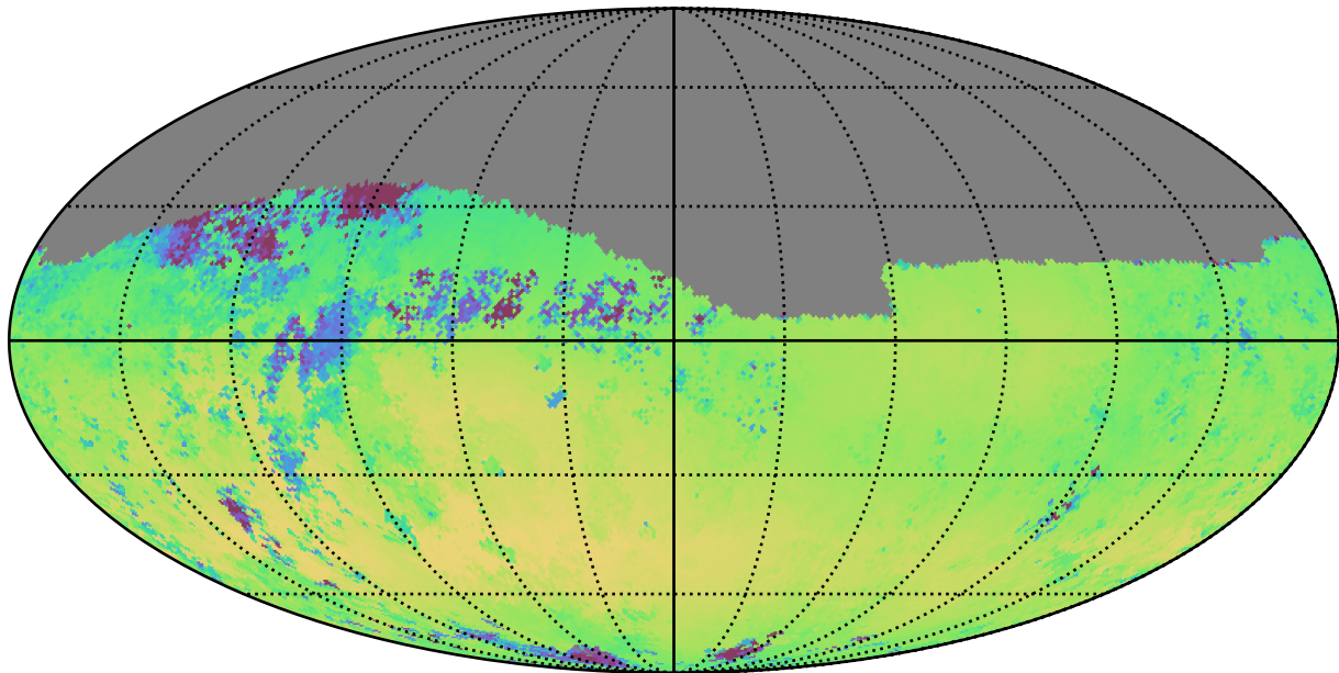
weather_cloudso20v3.4_10yrs Yr 1 r band: Median skyBrightness
