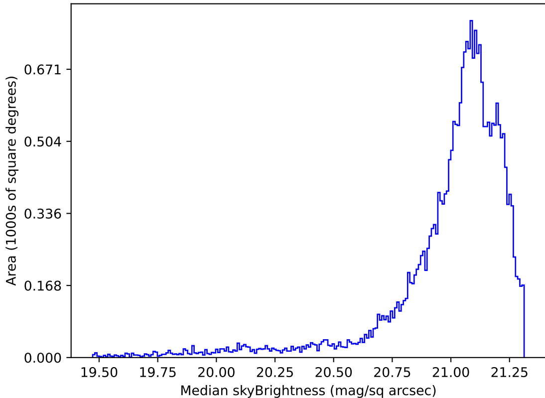
weather_cloudso20v3.4_10yrs Yr 1 r band: Median skyBrightness
