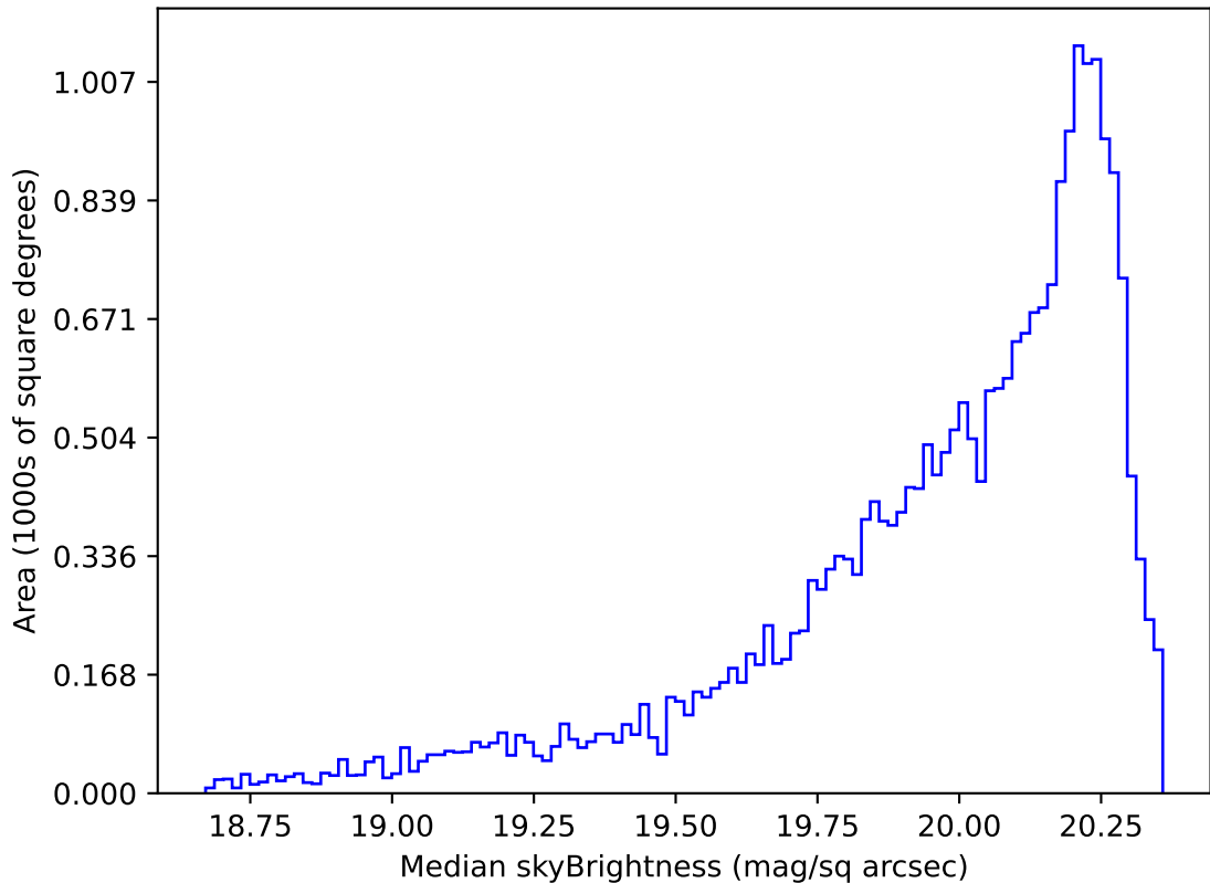
weather_cloudso20v3.4_10yrs Yr 1 i band: Median skyBrightness
