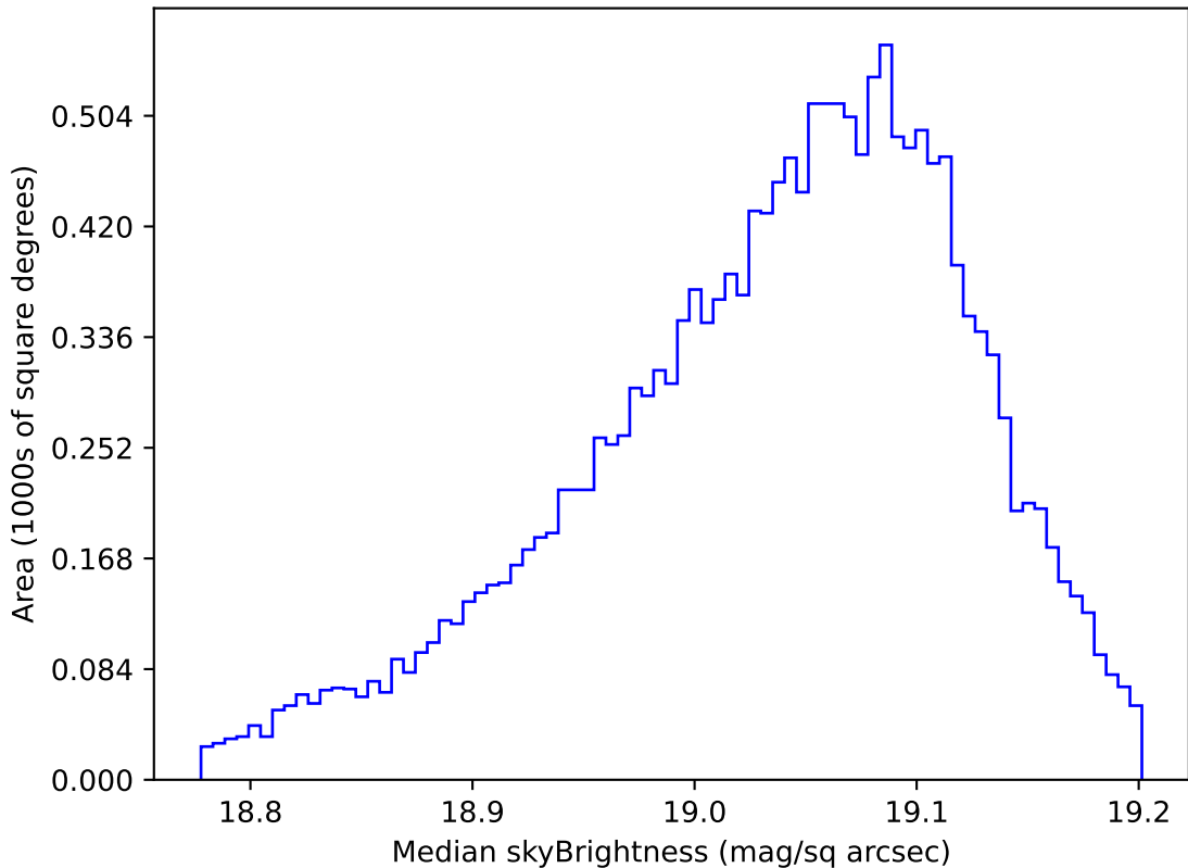
weather_cloudso20v3.4_10yrs WFD z band: Median skyBrightness
