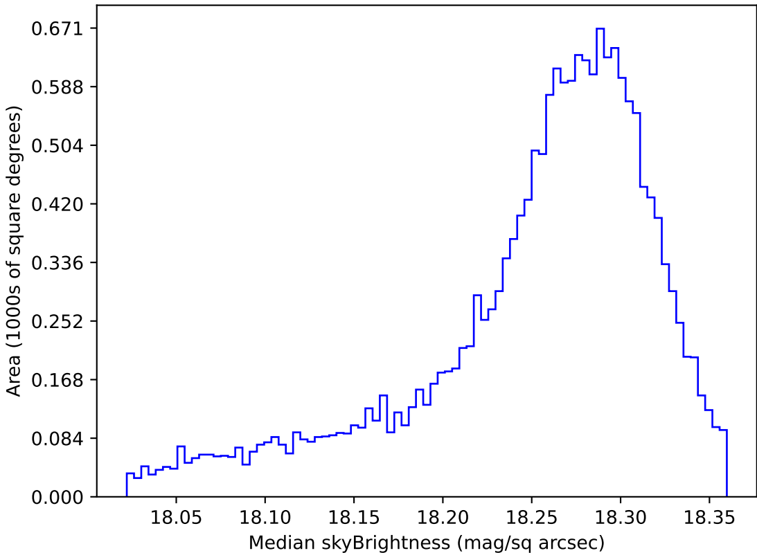
weather_cloudso20v3.4_10yrs WFD y band: Median skyBrightness
