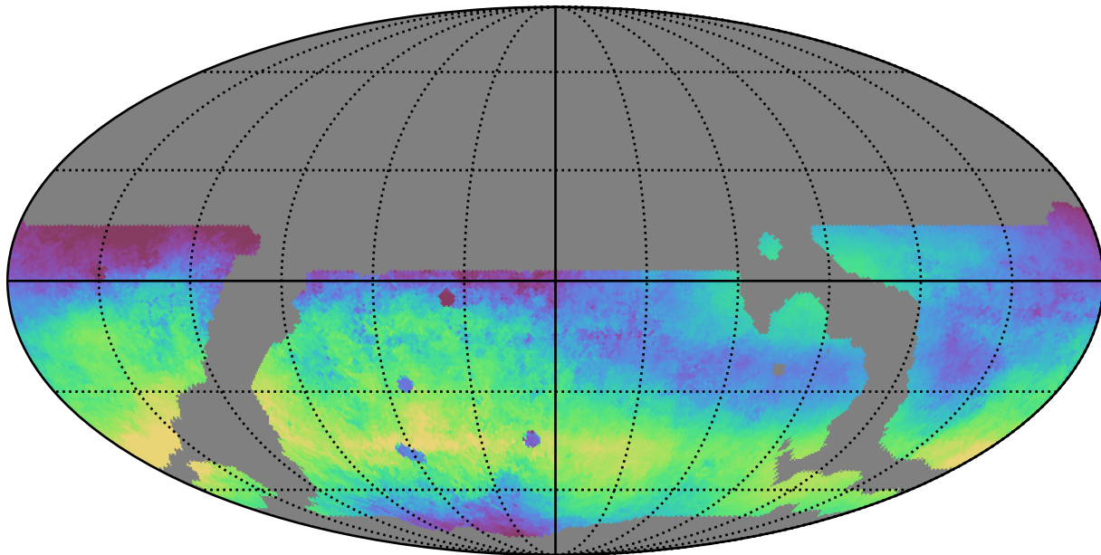
weather_cloudso20v3.4_10yrs WFD r band: Median skyBrightness
