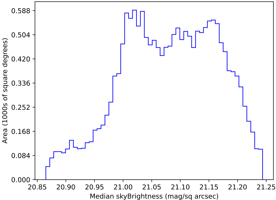
weather_cloudso20v3.4_10yrs WFD r band: Median skyBrightness
