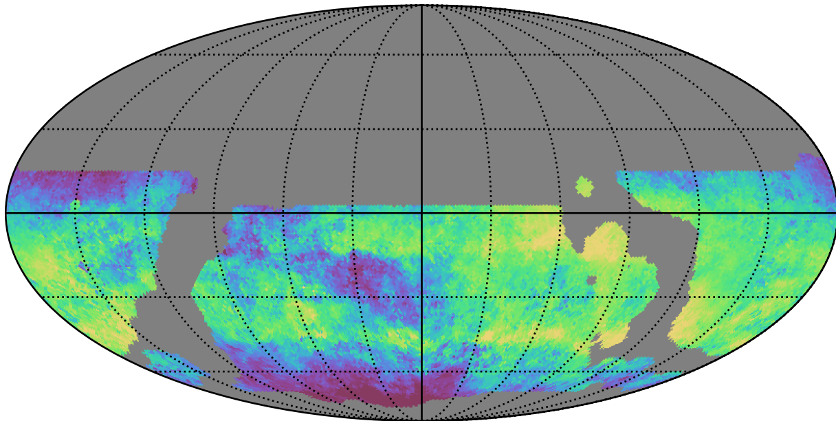
weather_cloudso20v3.4_10yrs WFD i band: Median skyBrightness
