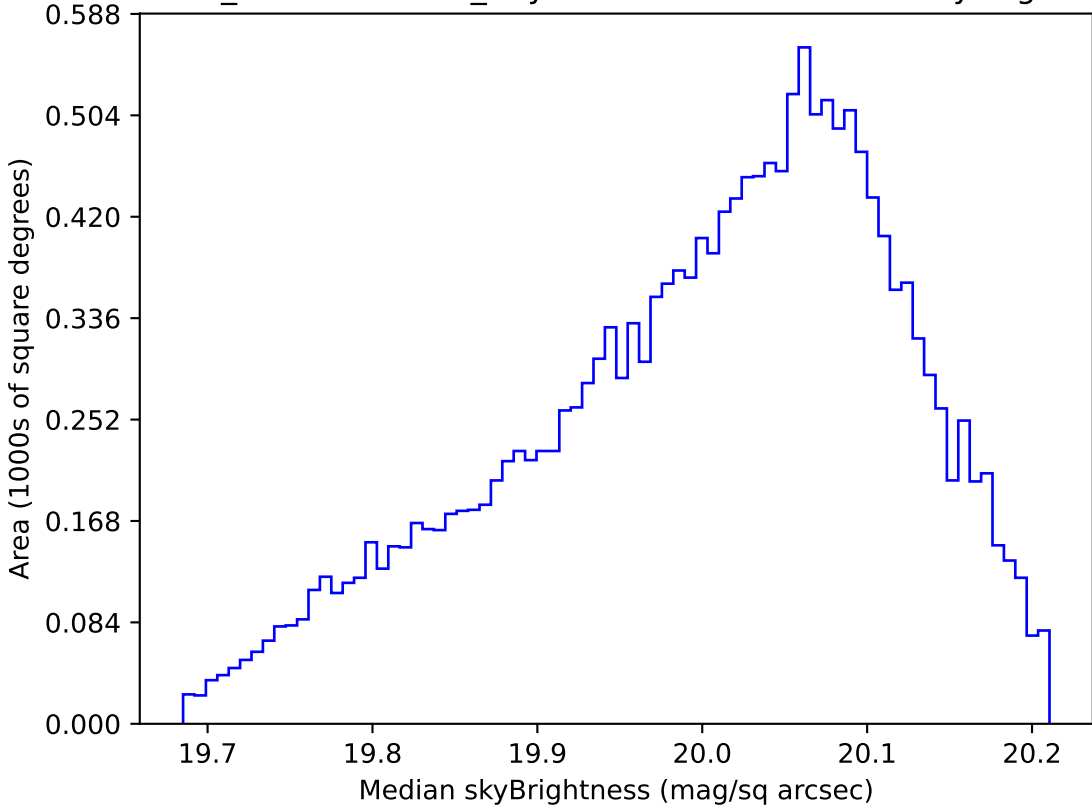
weather_cloudso20v3.4_10yrs WFD i band: Median skyBrightness
