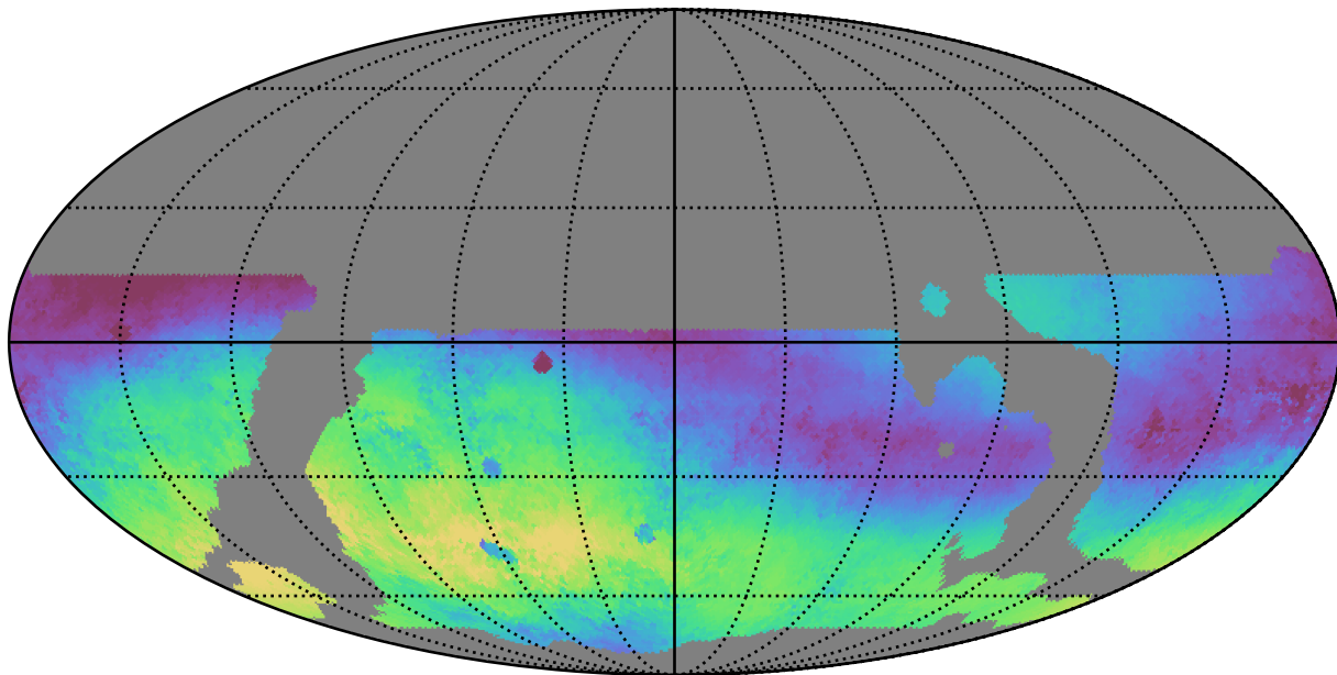
weather_cloudso20v3.4_10yrs WFD g band: Median skyBrightness
