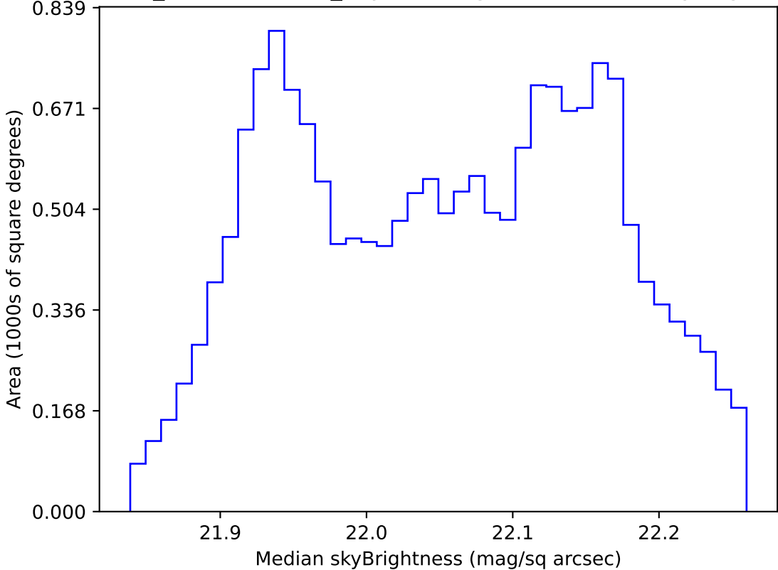
weather_cloudso20v3.4_10yrs WFD g band: Median skyBrightness
