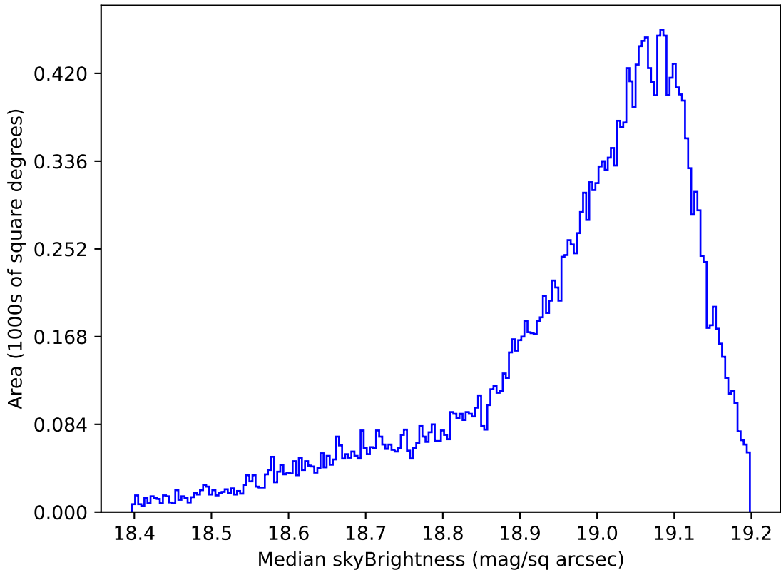
weather_cloudso20v3.4_10yrs All sky z band: Median skyBrightness
