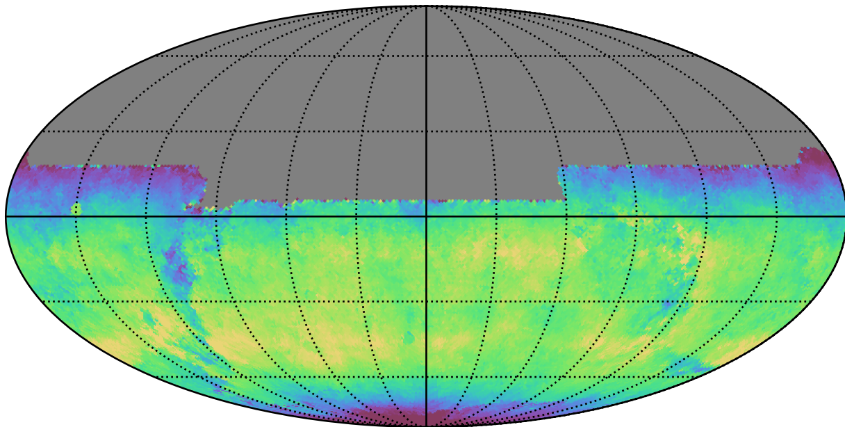
weather_cloudso20v3.4_10yrs All sky y band: Median skyBrightness
