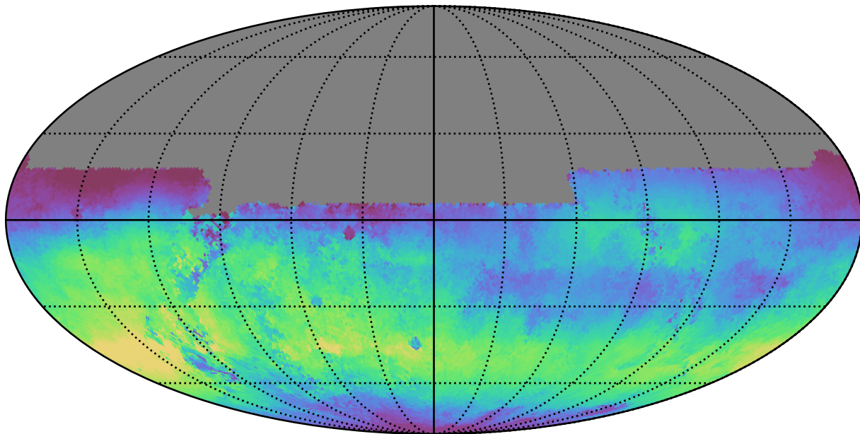
weather_cloudso20v3.4_10yrs All sky u band: Median skyBrightness
