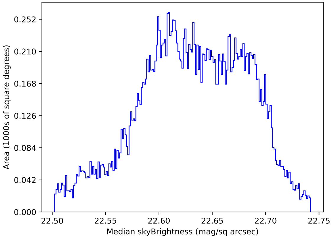
weather_cloudso20v3.4_10yrs All sky u band: Median skyBrightness
