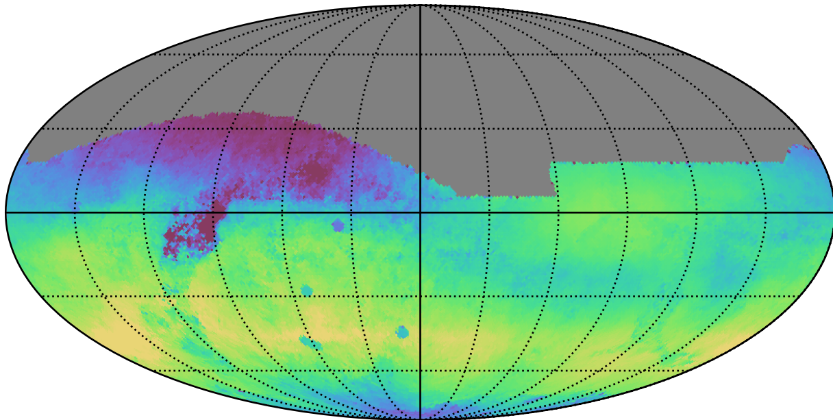
weather_cloudso20v3.4_10yrs All sky r band: Median skyBrightness
