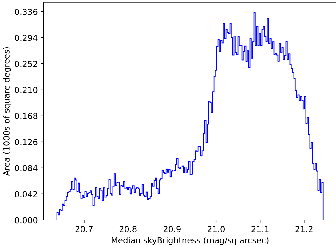
weather_cloudso20v3.4_10yrs All sky r band: Median skyBrightness
