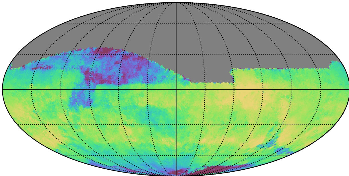
weather_cloudso20v3.4_10yrs All sky i band: Median skyBrightness
