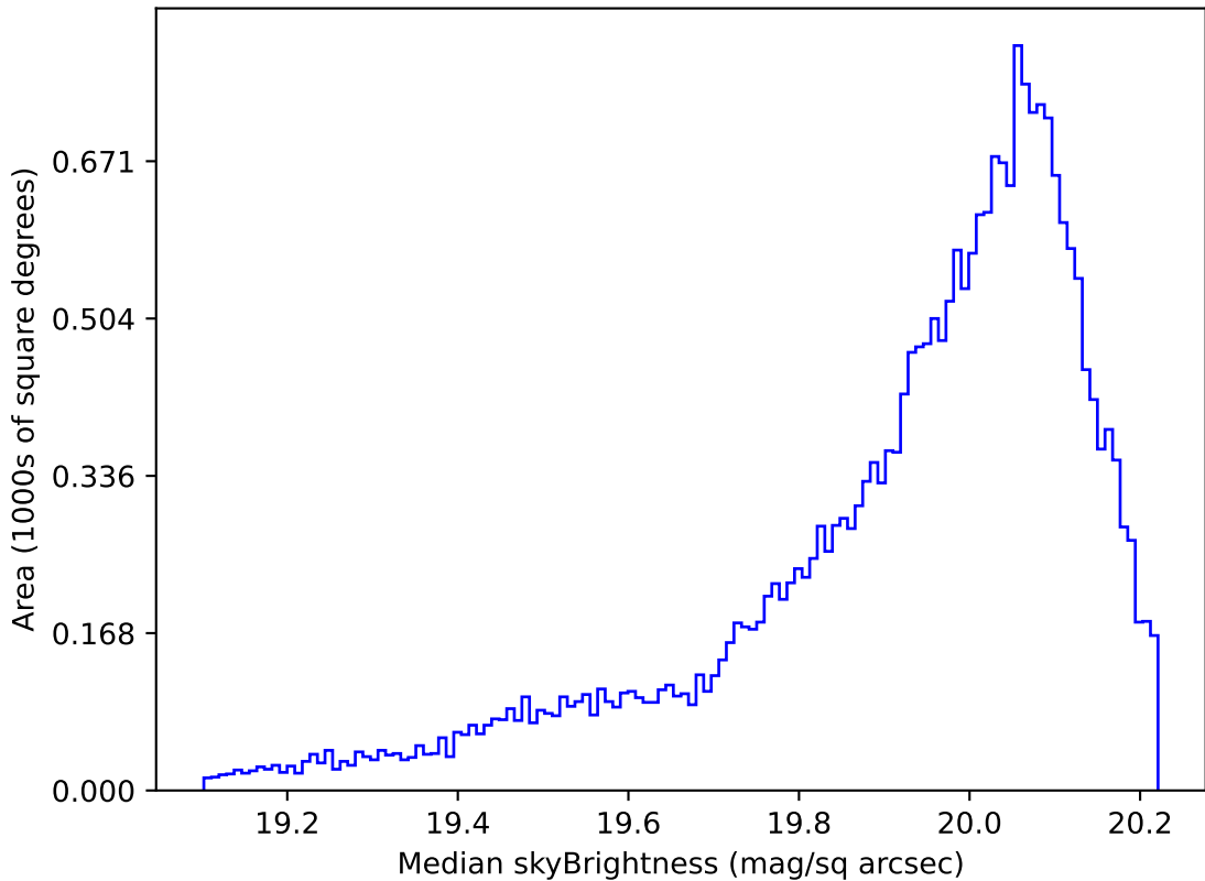
weather_cloudso20v3.4_10yrs All sky i band: Median skyBrightness
