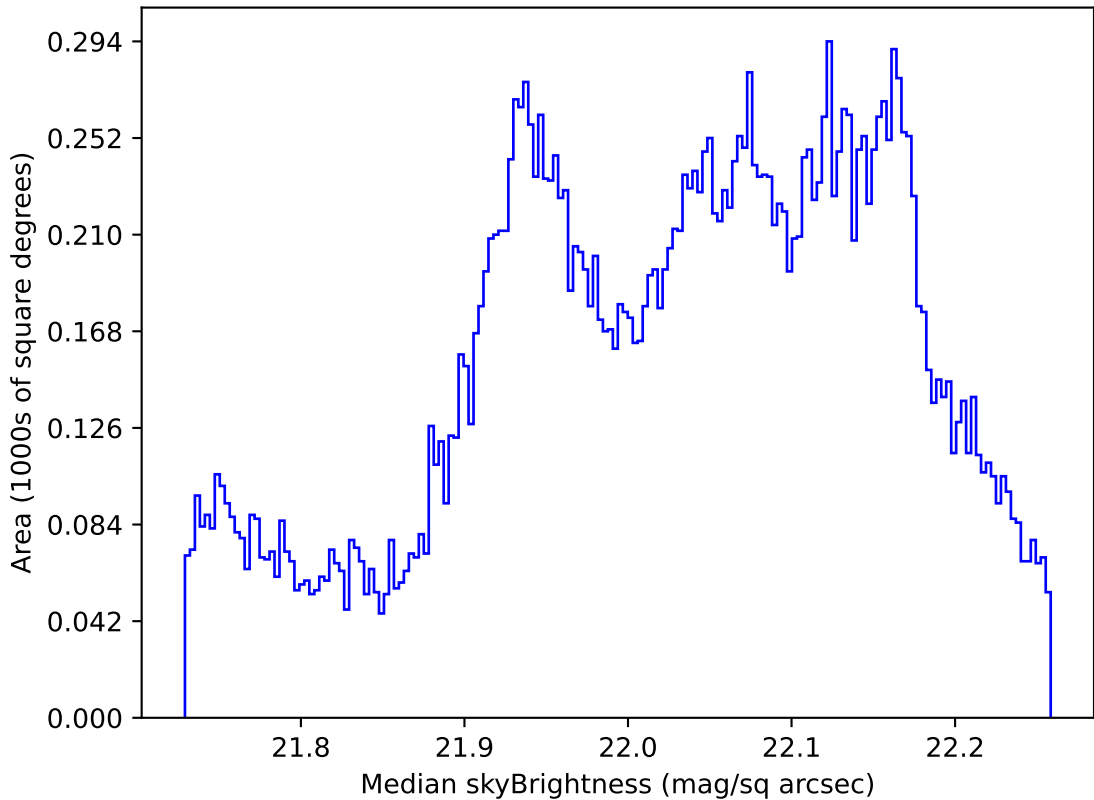
weather_cloudso20v3.4_10yrs All sky g band: Median skyBrightness
