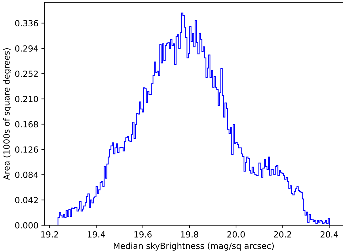
weather_cloudso20v3.4_10yrs All sky all bands: Median skyBrightness
