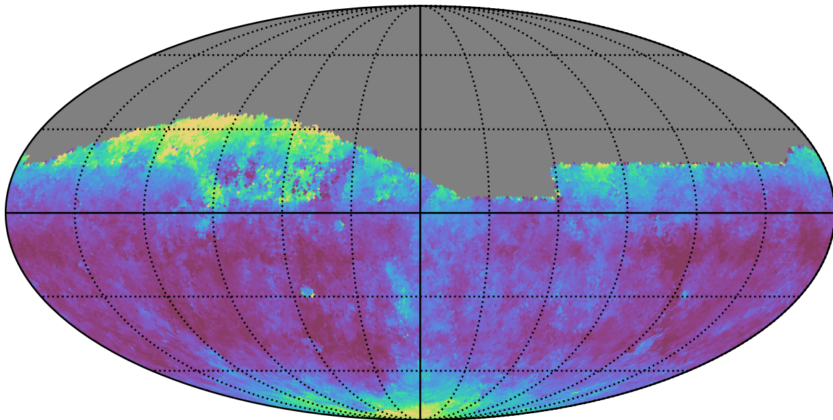
weather_cloudso20v3.4_10yrs Yr 1 all bands: Median seeingGeom
