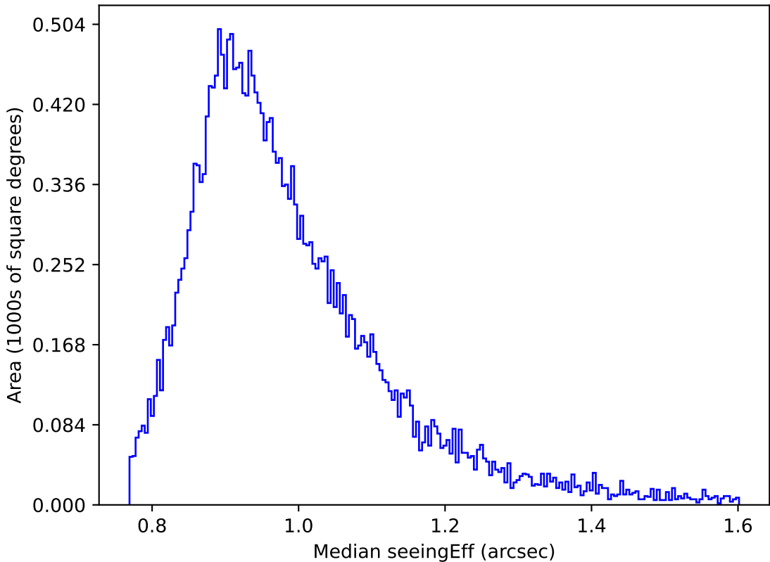
weather_cloudso20v3.4_10yrs Yr 1 z band: Median seeingEff
