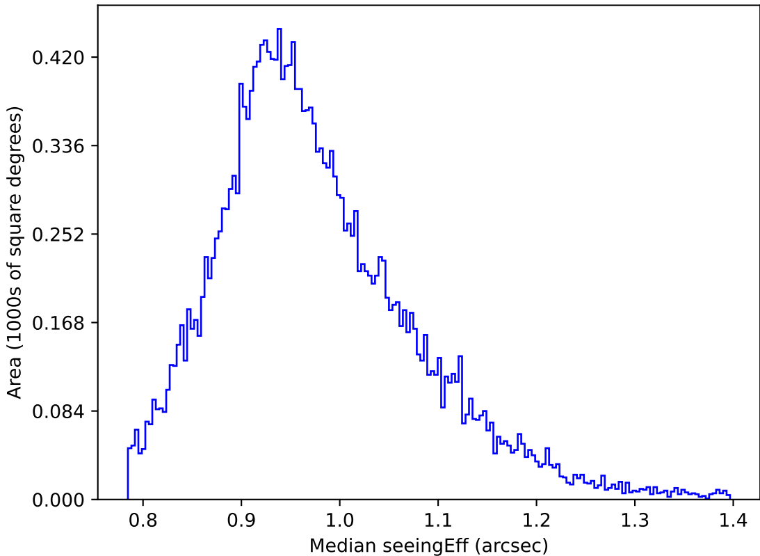
weather_cloudso20v3.4_10yrs Yr 1 y band: Median seeingEff
