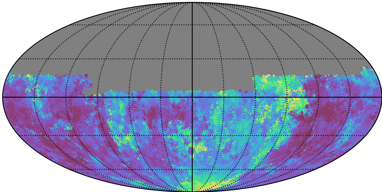
weather_cloudso20v3.4_10yrs Yr 1 u band: Median seeingEff
