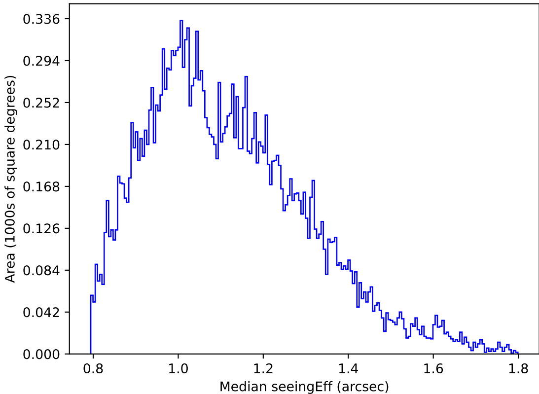
weather_cloudso20v3.4_10yrs Yr 1 u band: Median seeingEff
