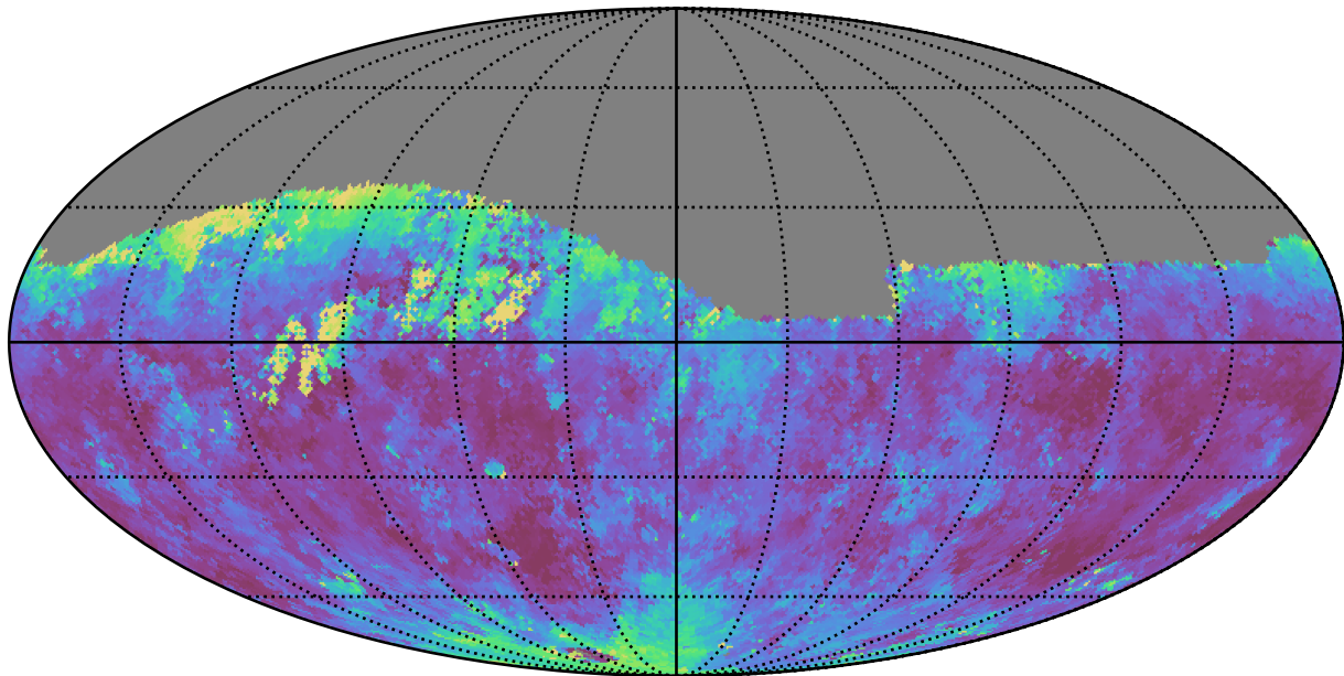
weather_cloudso20v3.4_10yrs Yr 1 r band: Median seeingEff
