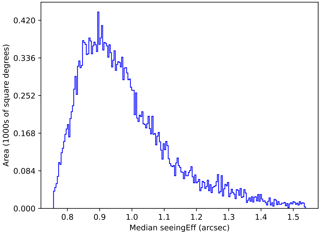
weather_cloudso20v3.4_10yrs Yr 1 r band: Median seeingEff
