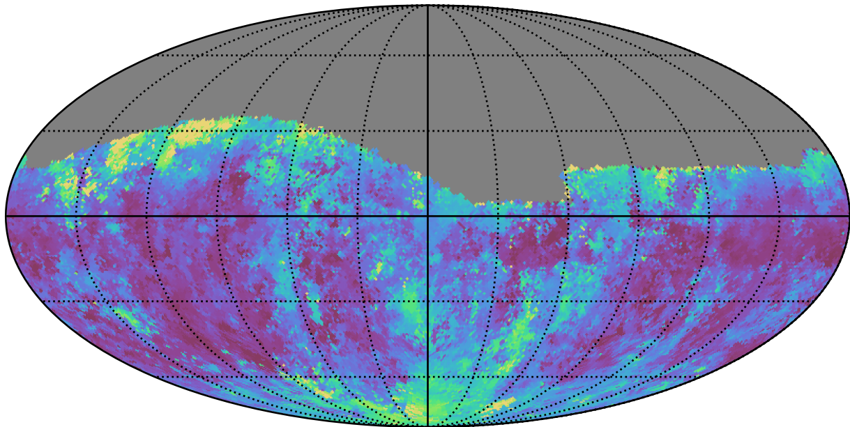
weather_cloudso20v3.4_10yrs Yr 1 g band: Median seeingEff
