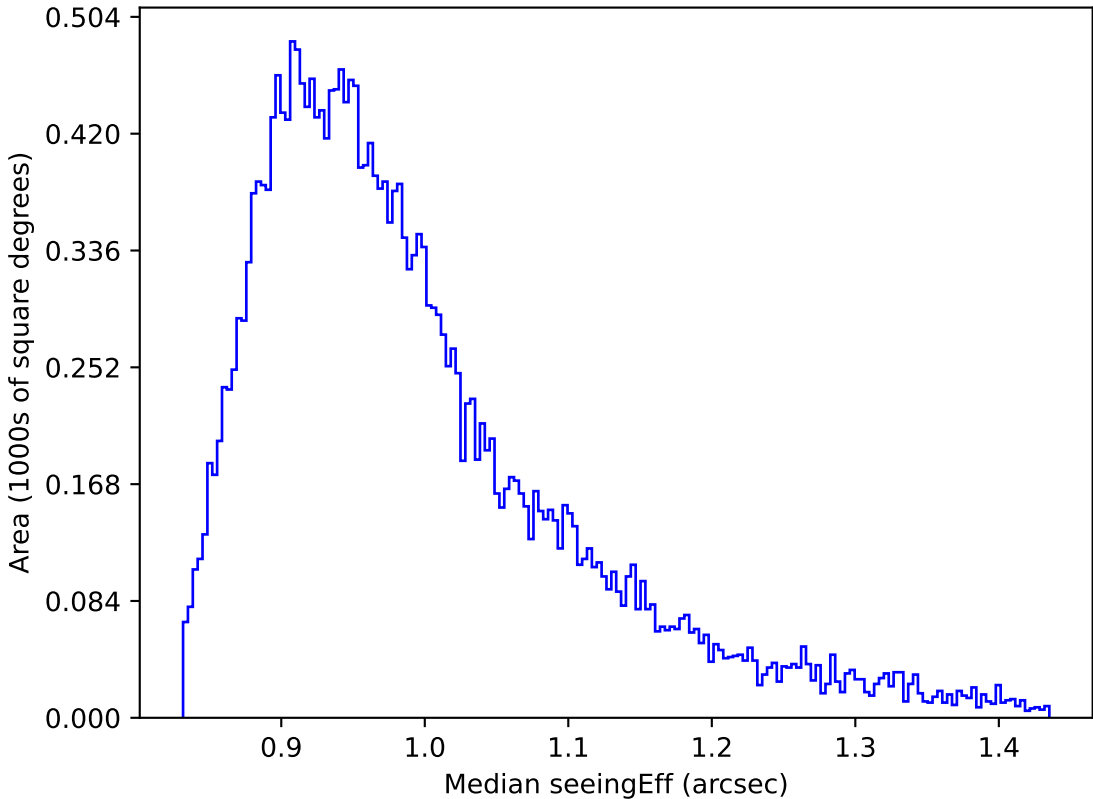
weather_cloudso20v3.4_10yrs Yr 1 all bands: Median seeingEff
