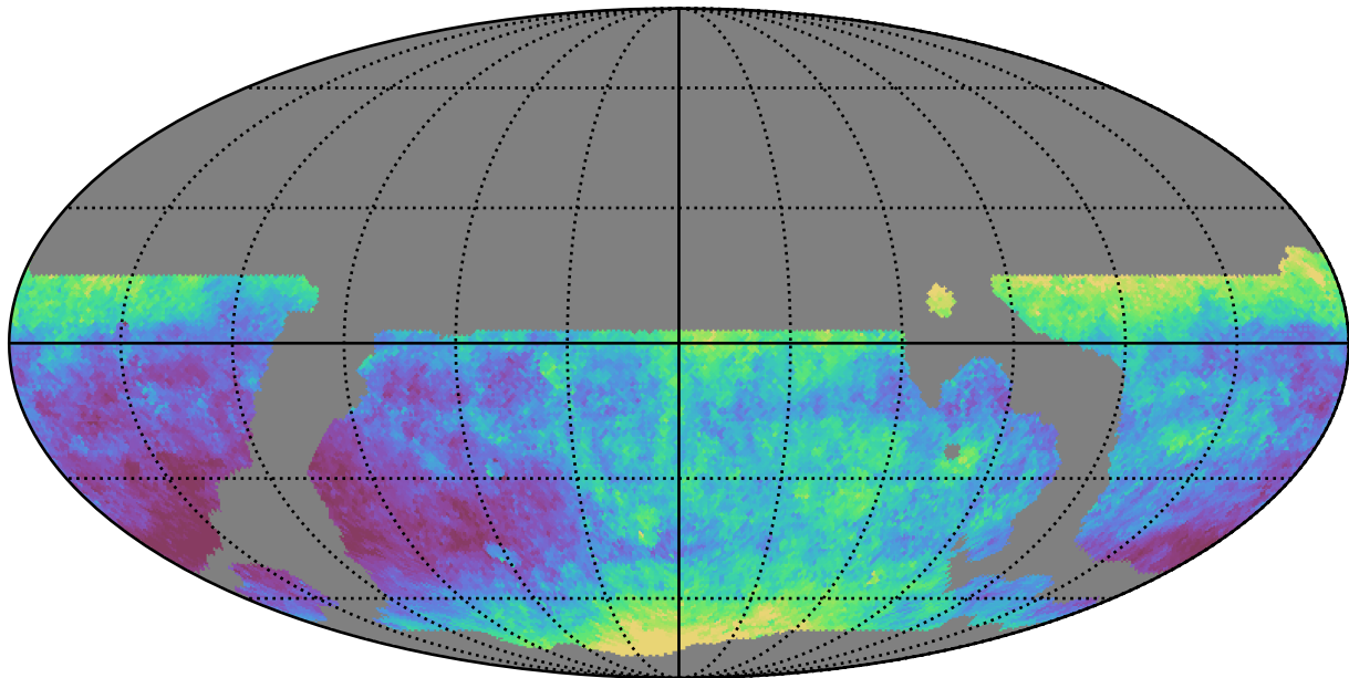
weather_cloudso20v3.4_10yrs WFD z band: Median seeingEff
