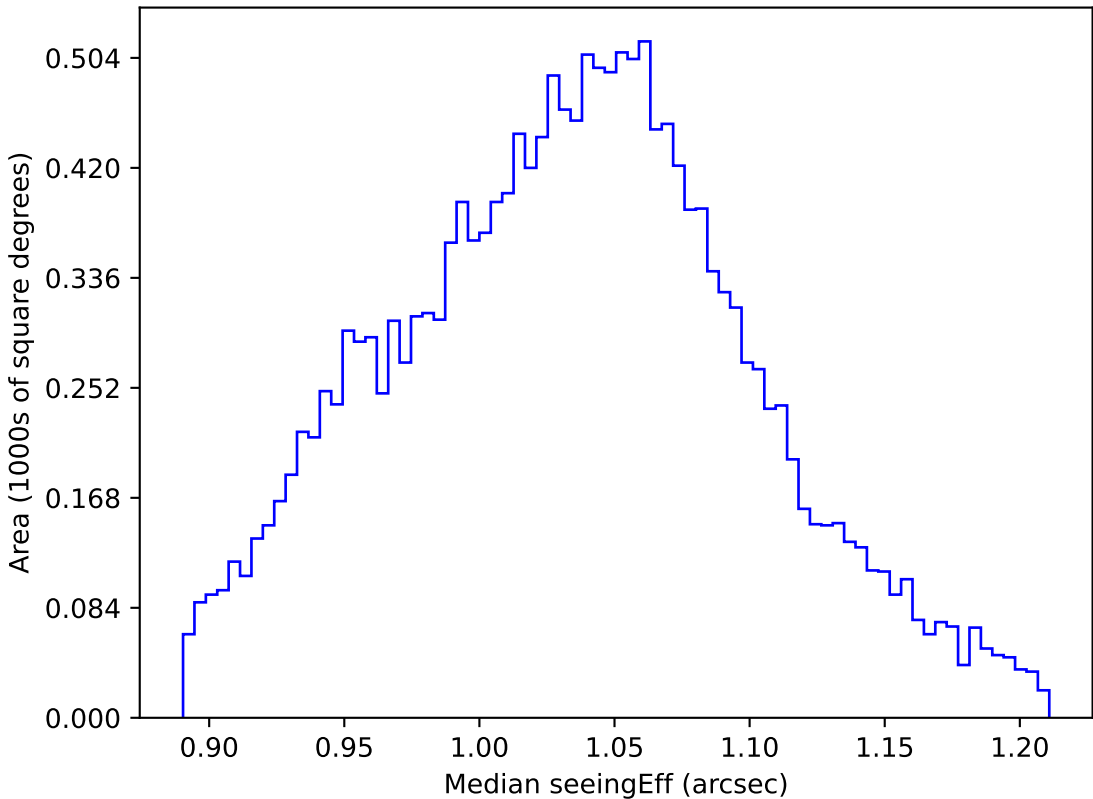
weather_cloudso20v3.4_10yrs WFD z band: Median seeingEff
