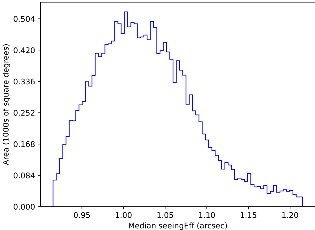
weather_cloudso20v3.4_10yrs WFD y band: Median seeingEff
