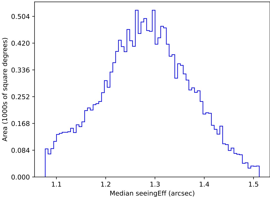
weather_cloudso20v3.4_10yrs WFD u band: Median seeingEff
