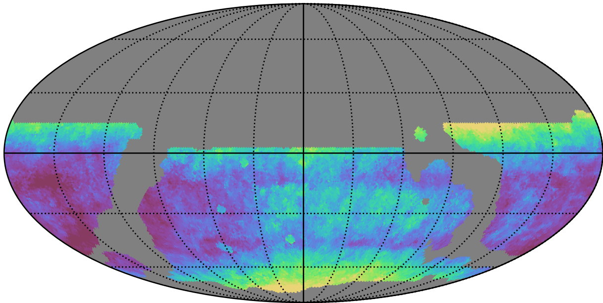
weather_cloudso20v3.4_10yrs WFD r band: Median seeingEff
