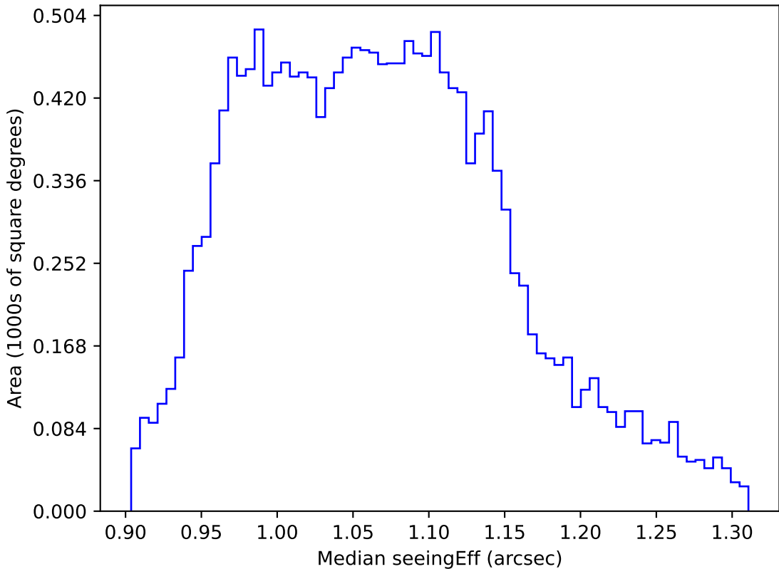
weather_cloudso20v3.4_10yrs WFD r band: Median seeingEff
