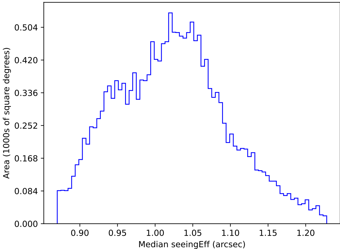
weather_cloudso20v3.4_10yrs WFD i band: Median seeingEff
