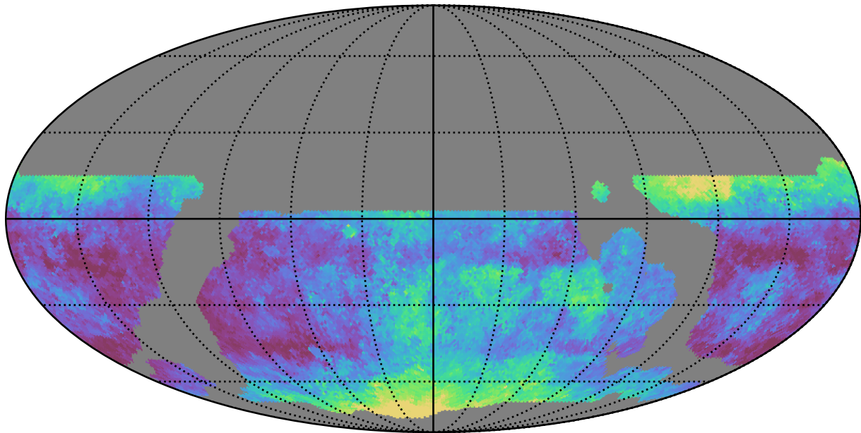
weather_cloudso20v3.4_10yrs WFD g band: Median seeingEff
