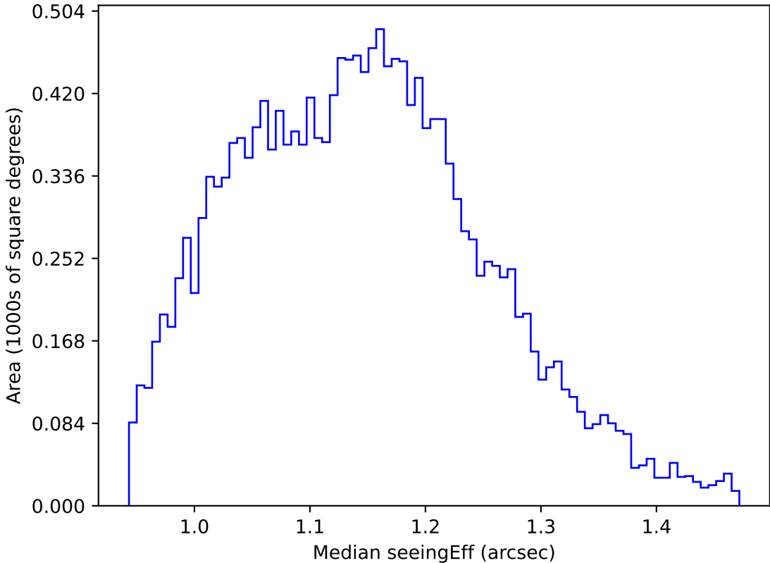
weather_cloudso20v3.4_10yrs WFD g band: Median seeingEff
