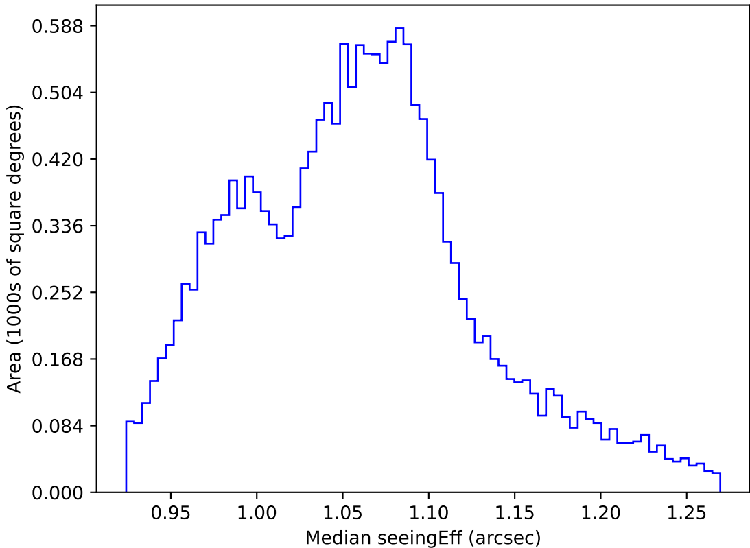
weather_cloudso20v3.4_10yrs WFD all bands: Median seeingEff
