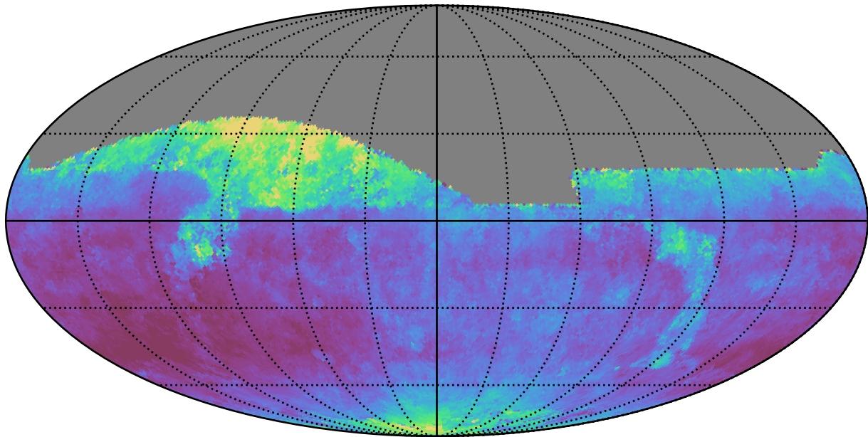
weather_cloudso20v3.4_10yrs All sky z band: Median seeingEff
