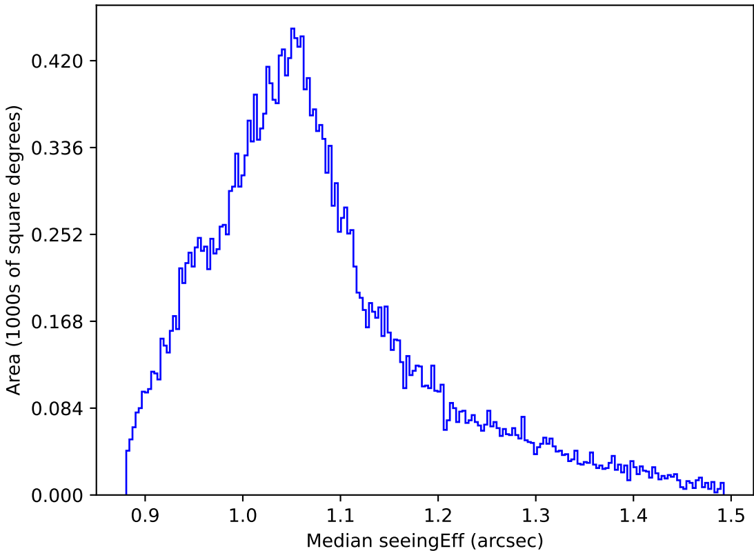
weather_cloudso20v3.4_10yrs All sky z band: Median seeingEff
